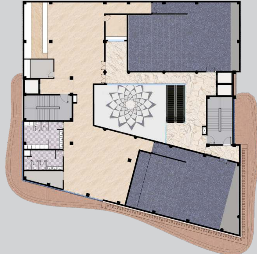
Plan View : 4th and 5th Floor (18,449 Sq ft)
