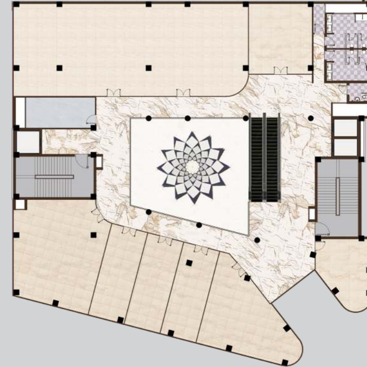
Plan View: 1st and 2nd Floor (23,164 Sq ft)
