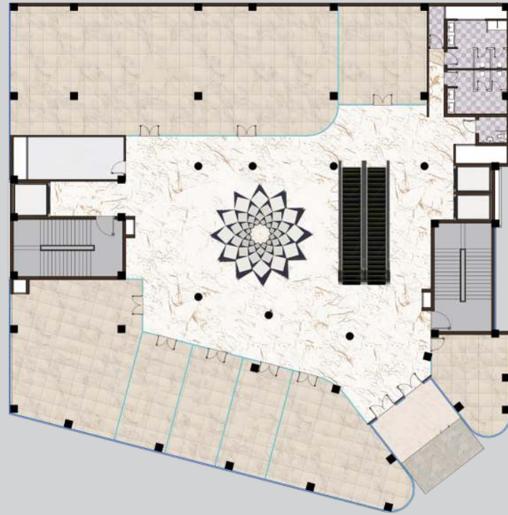
Plan View: Ground Floor (14,122 Sq ft)
